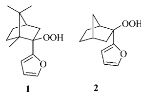
Figure 2. ( R )-Camphor- and ( S )-norcamphor-derived hydroperoxides.
