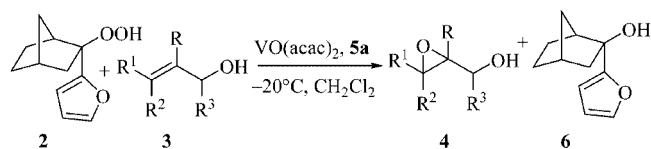
Scheme 2. Asymmetric epoxidation with \text{VO}(\text{acac})_2/\mathbf{5a} and hydroperoxide 2 .
