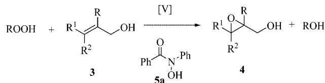
Scheme 1. Vanadium-catalyzed epoxidation of allylic alcohols.
