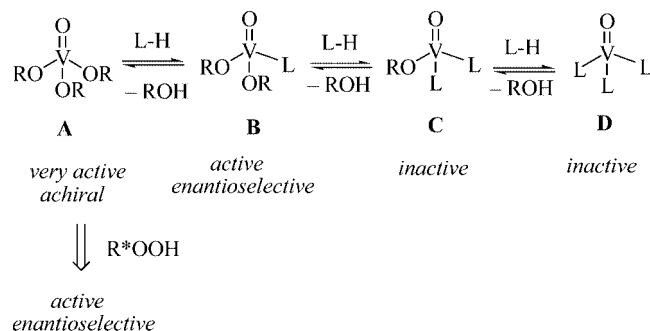
Figure 3. Vanadium/ligand complexation equilibria.
